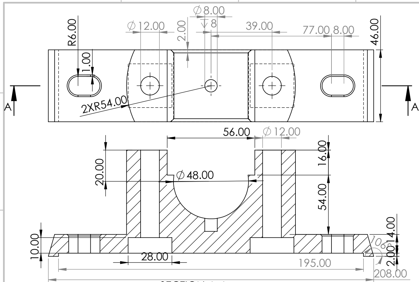
Casting SECTION A-A SCALE 1 : 1.5
